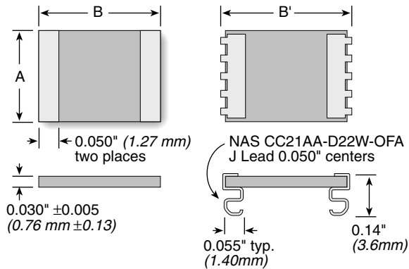
With J-bend Option:
